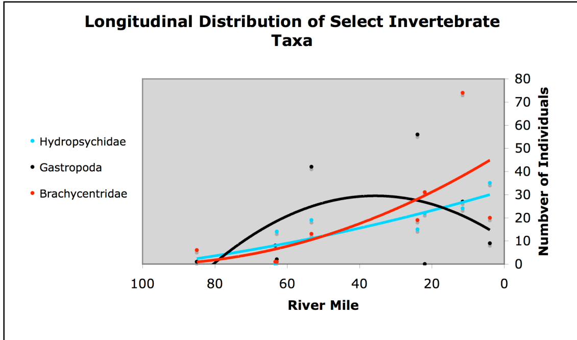
Figure 12. Representative taxa reflecting the predictions of the RCC. Hydropsychids and brachycentrids are primarily collectors; consistent with the RCC, their numbers smoothly increase in the downstream direction. Gastropods are largely grazers and hence rely heavily on periphyton; thus, their peak abundances in the middle reaches also conform to the RCC.
