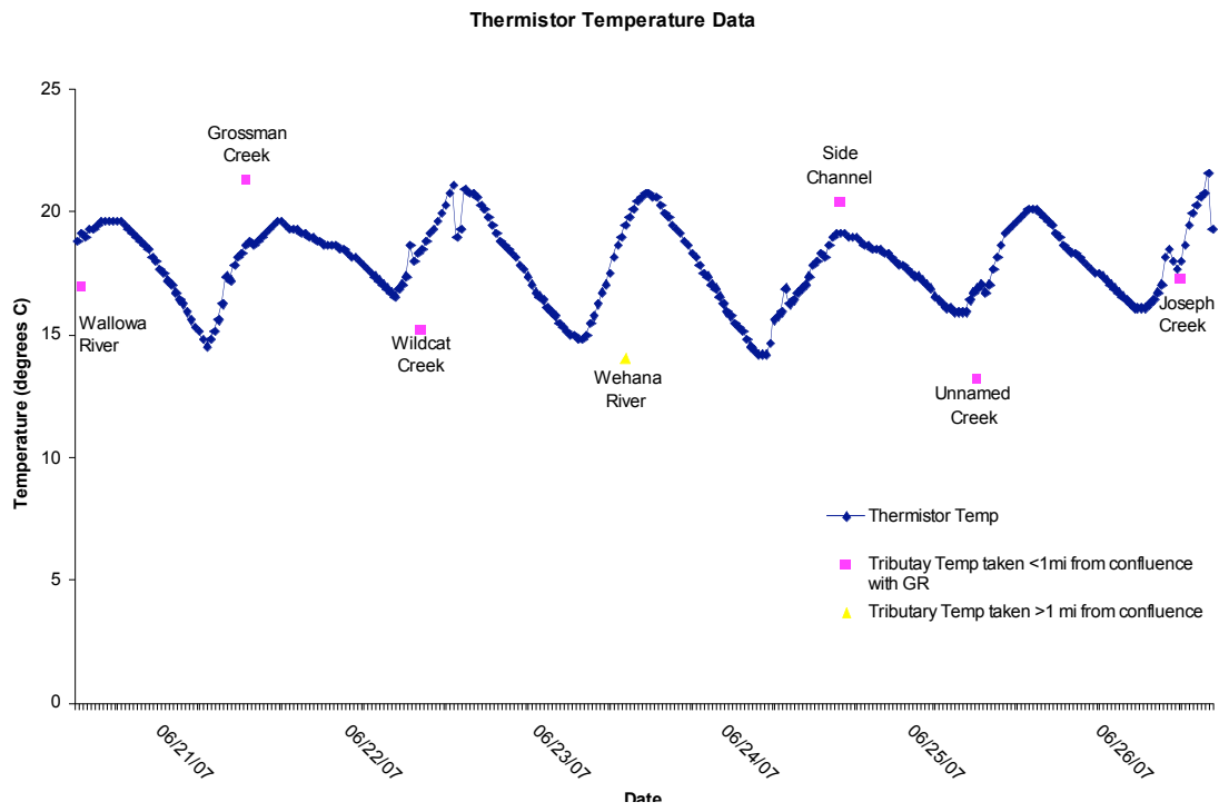
Figure 3. Thermistor temperature data
