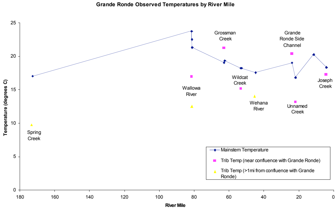
Figure 1 Temperature variations observed along the Grande Ronde River between 06/19/07 and 06/26/07 plotted against river mile. The measurements at the tributaries and along the mainstem Grande Ronde were taken at approximately the same time of day and thus are subject to the same diurnal variations. Thus this plot is most useful for determining the influence that each tributary has on the mainstem.
